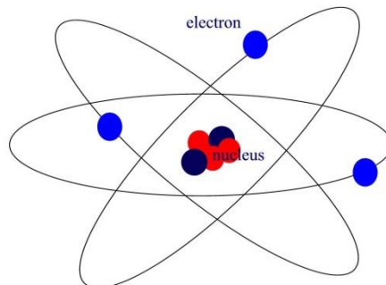
Atomic Planetary Model
